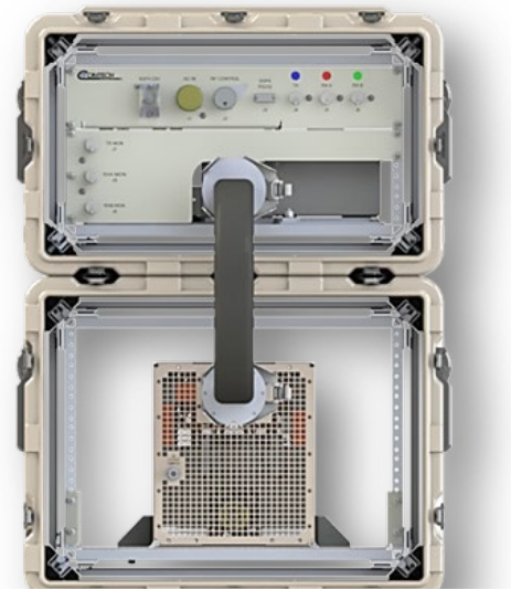
Figure 12 C-Band Filter Case and 500 Watt SSPA
