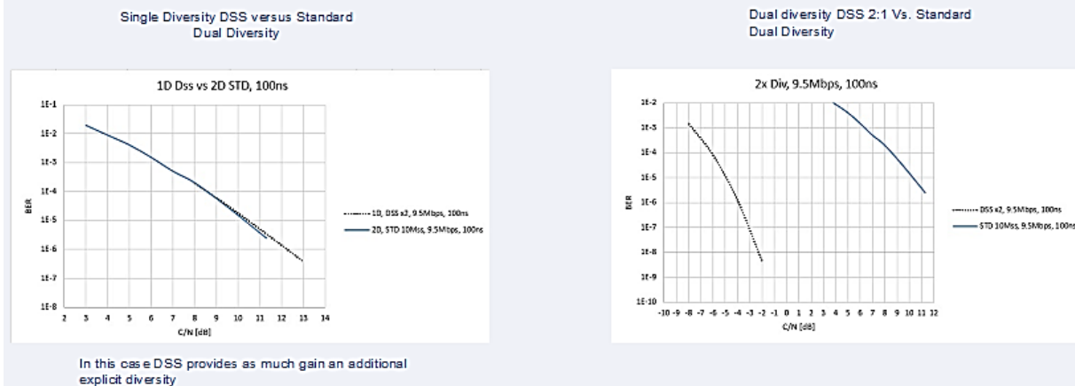
Figure 3 Standard Diversity comparison to DSSS Diversity
