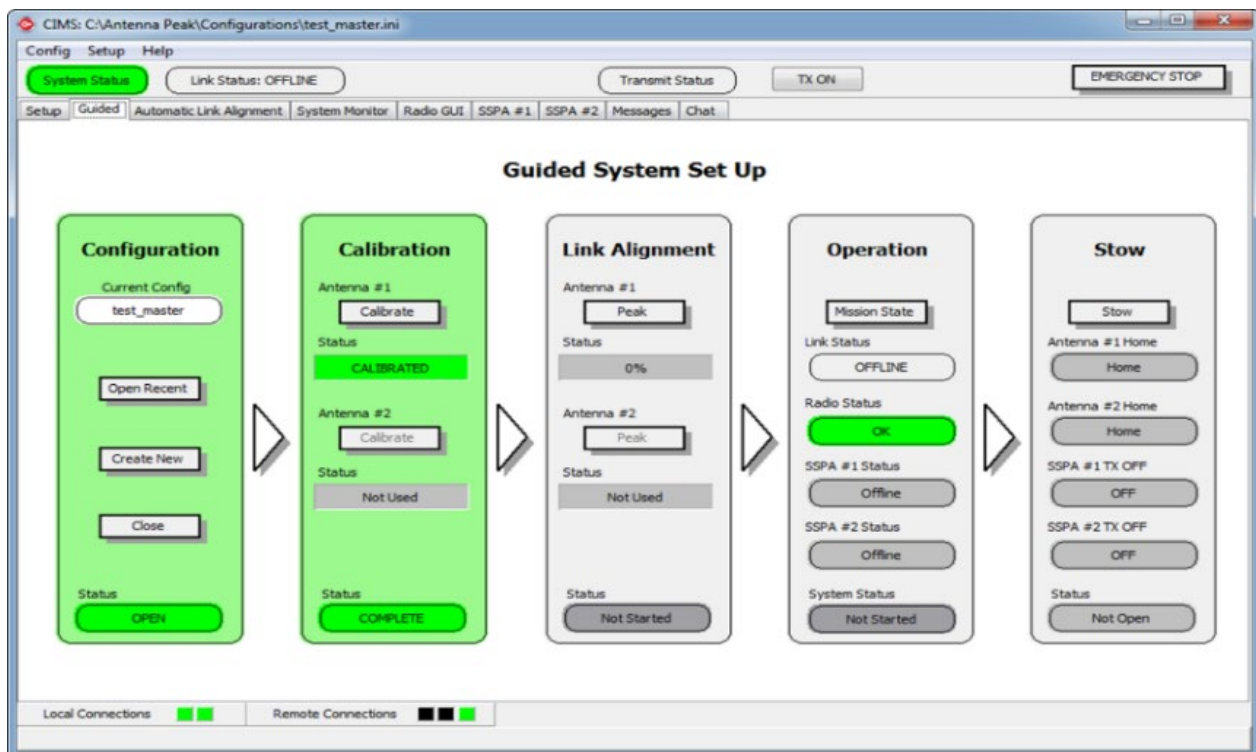
Figure 15 CIMS Guided Setup Screen
