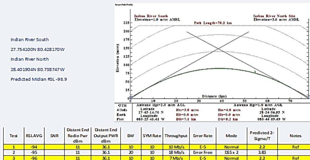
Figure 4 DSSS Performance in Real World Conditions
